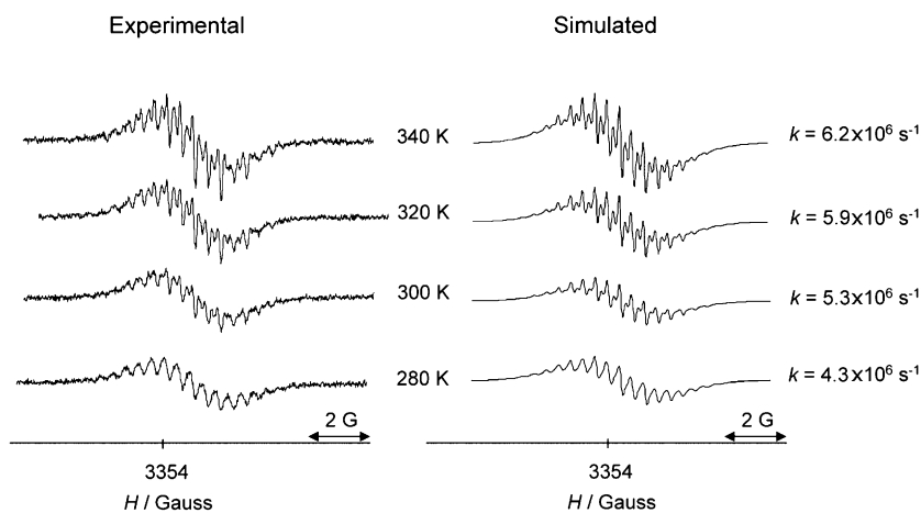
Figure 4. Experimental (left) and simulated (right) EPR spectra of the mixed valence species 1^{\cdot-} at different temperatures in DMSO/benzonitrile (45:55) and 0.15 M [NnBu_4]PF_6 .
