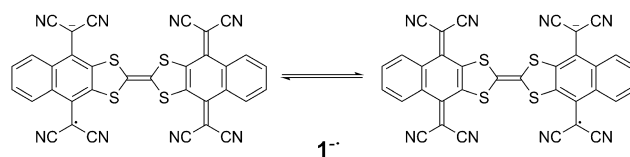
Scheme 2. Thermally activated IET process in 1^{\cdot-} .
